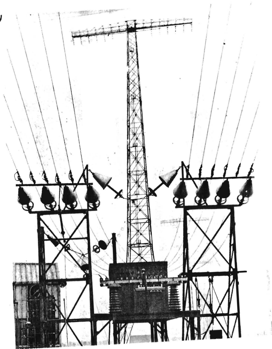
View at Rocky Point transmitting station. Download terminations for one longwave antenna in foreground, towers of second longwave antenna in background.
