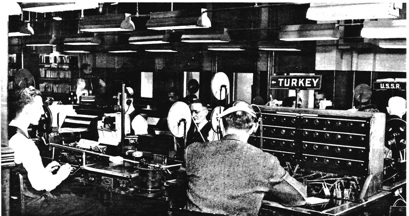
Section of terminal operating office of R.C.A. Communications, New York City. Foreground shows radiotelegraph concentrator position for switching of non-continuous circuits to active operating positions.
