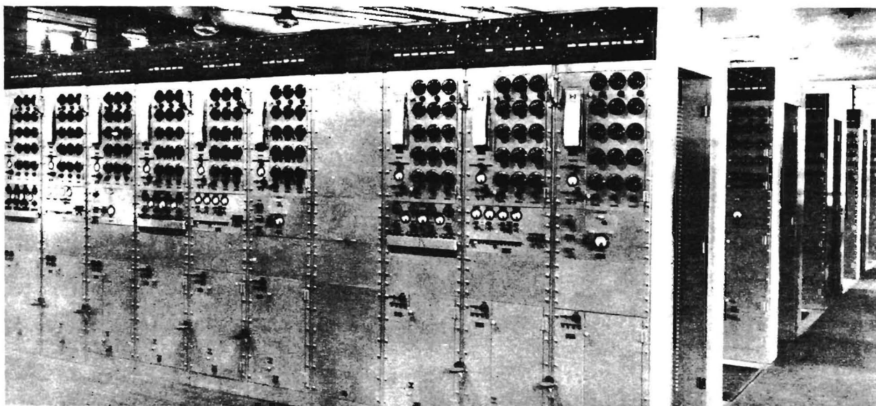
View of one section of receiver room in main shortwave receiving building of R.C.A. Communications receiving station, Riverhead, New York, showing in foreground three complete three-set diversity receiver groups and ends of 11 rows of such receiver groups.
