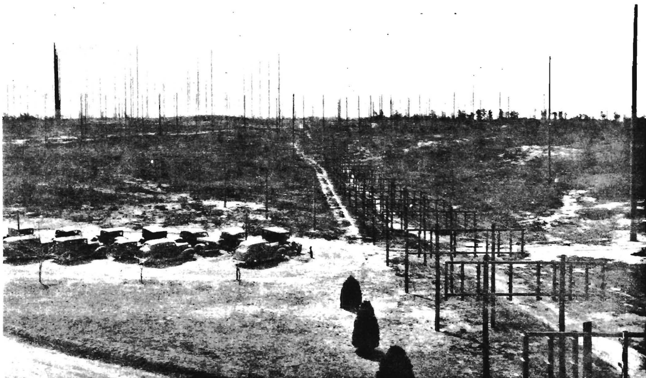
View from front of main receiving building at Riverhead showing one of the transmission line trunk systems and more of the antenna poles.
