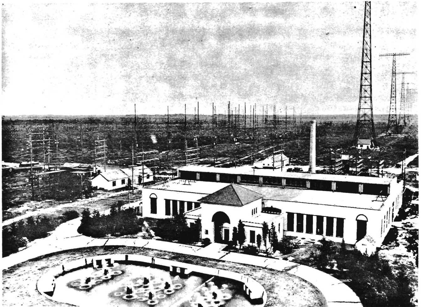
Main Transmitter Building, at R.C.A. Communications transmitting station, Rocky Point, New York. Also shows one of the longwave antennas and a few of the short-wave antennas.
