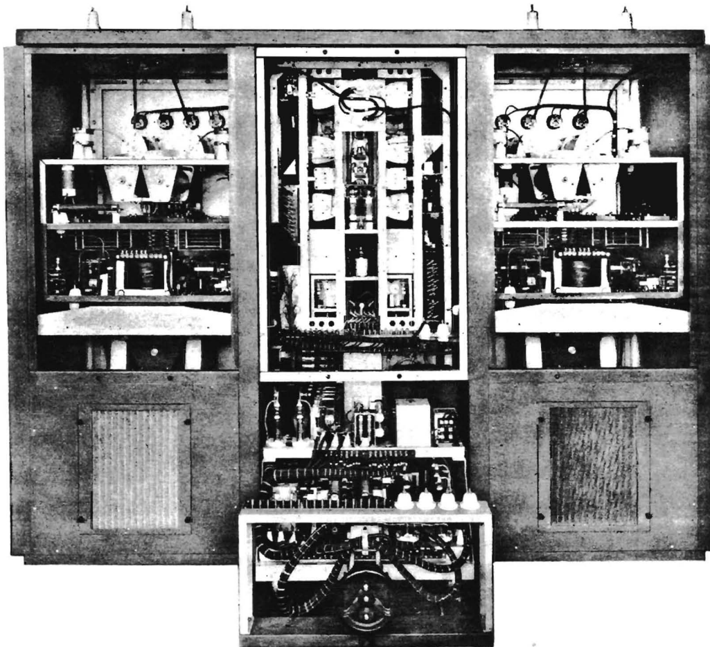
2-CHANNEL 5 KW 2.5/20 MC GENERAL COMMUNICATION TRANSMITTER. TE 308-C
