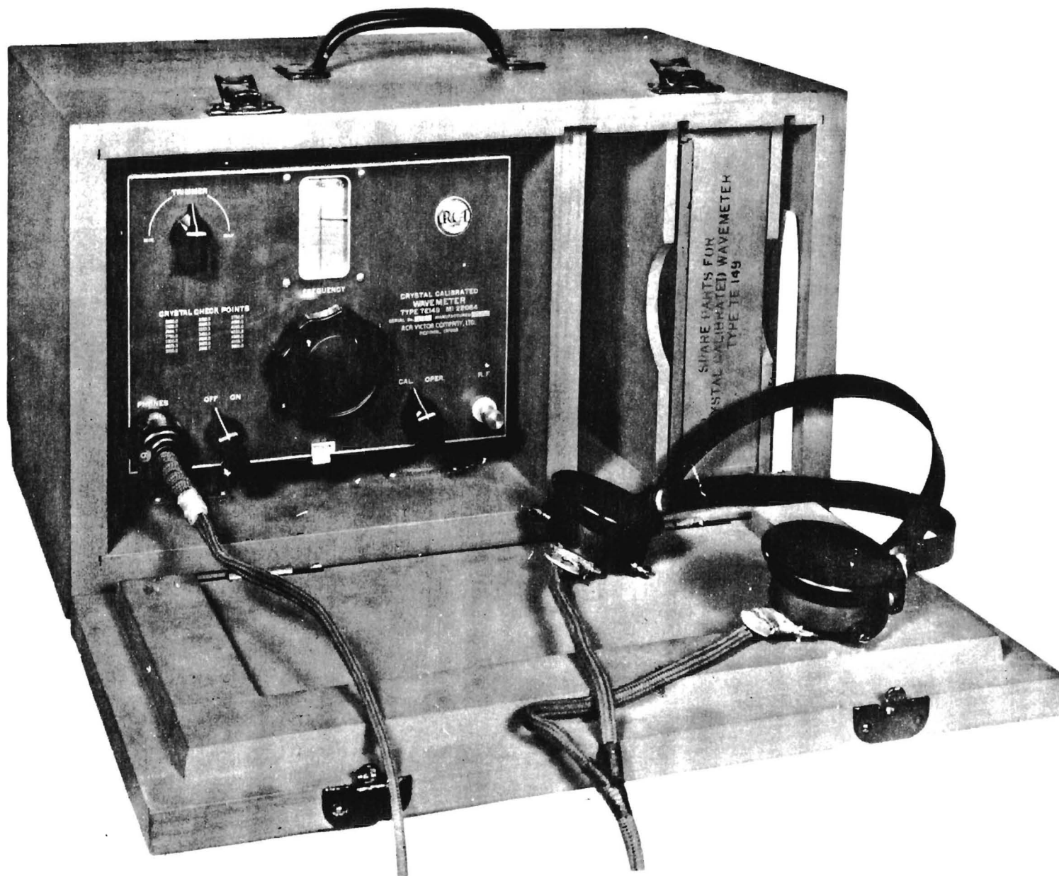
CRYSTAL CALIBRATED FREQUENCY METER EQUIPMENT. TE 149
